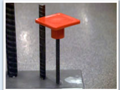
Steel-reinforced cap
